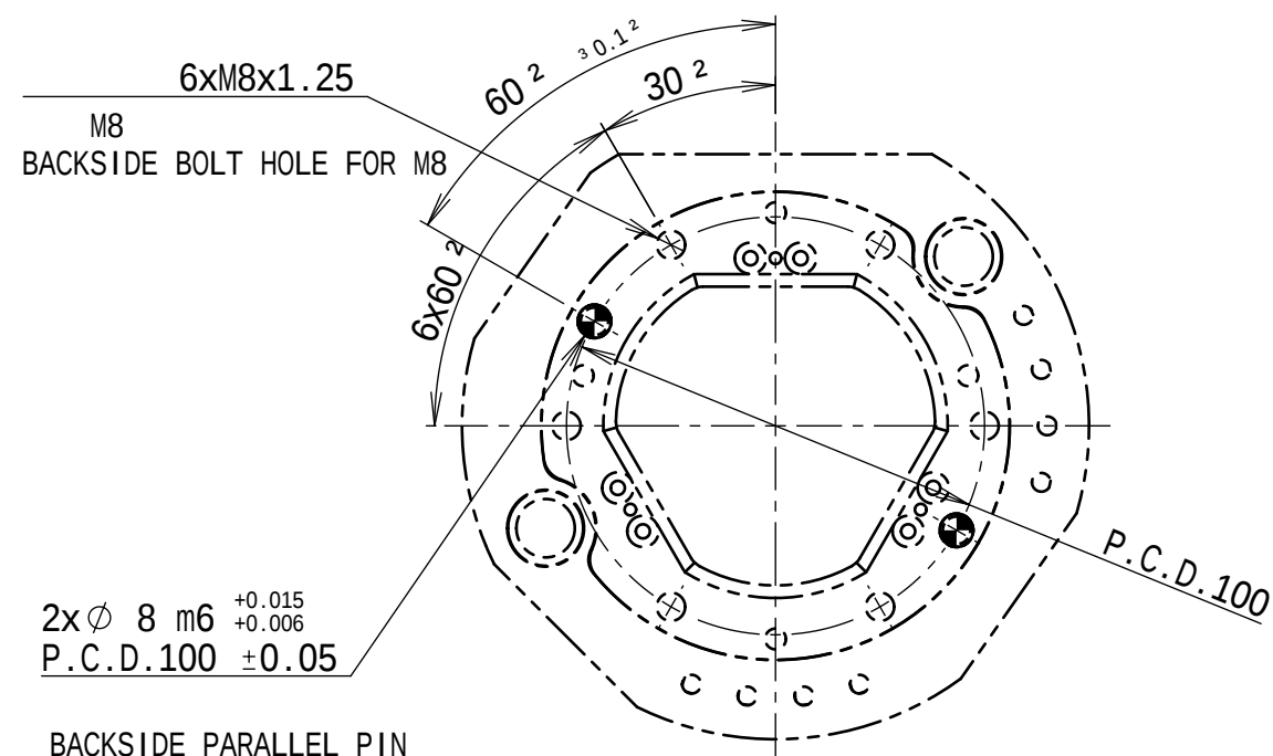
A VIEW A : CONNECTING DIMENSION VIEW
