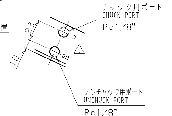
(B 矢視図) VIEW B
