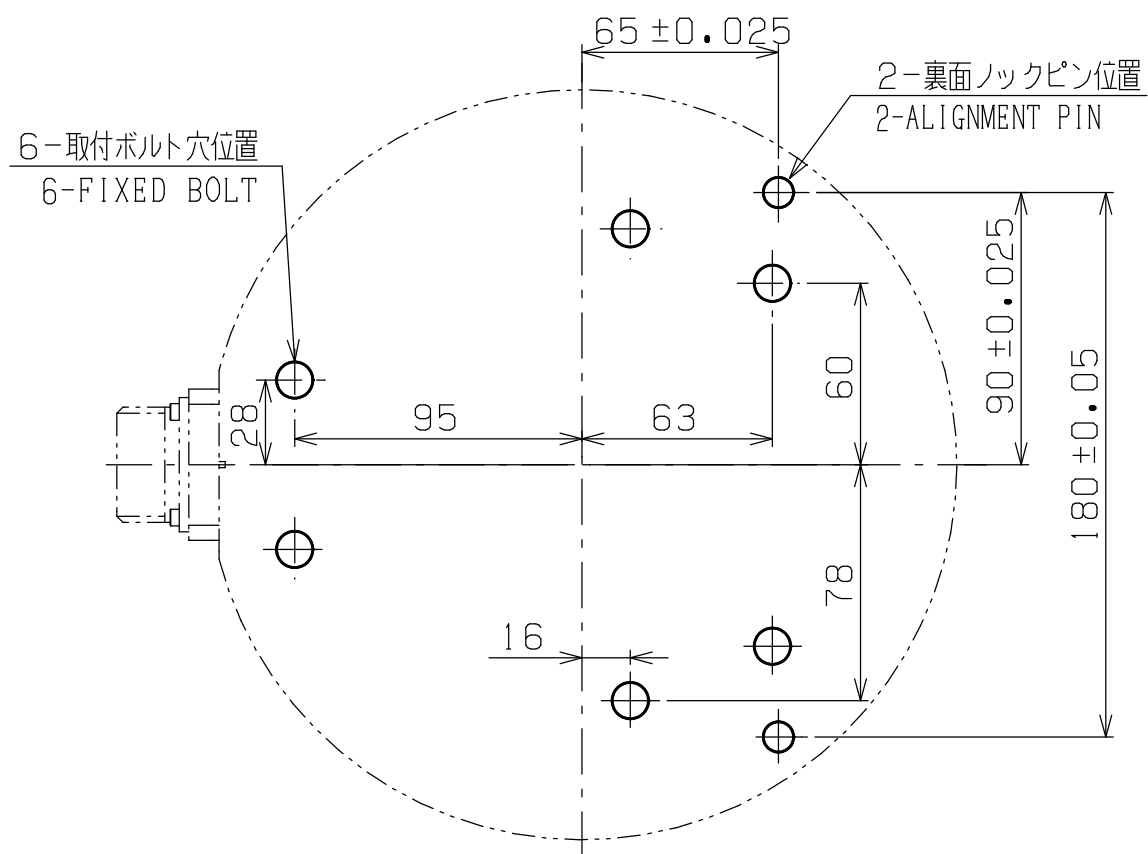
取合寸法図 (A矢視) CONNECTING DIMENSION VIEW (VIEW A)
