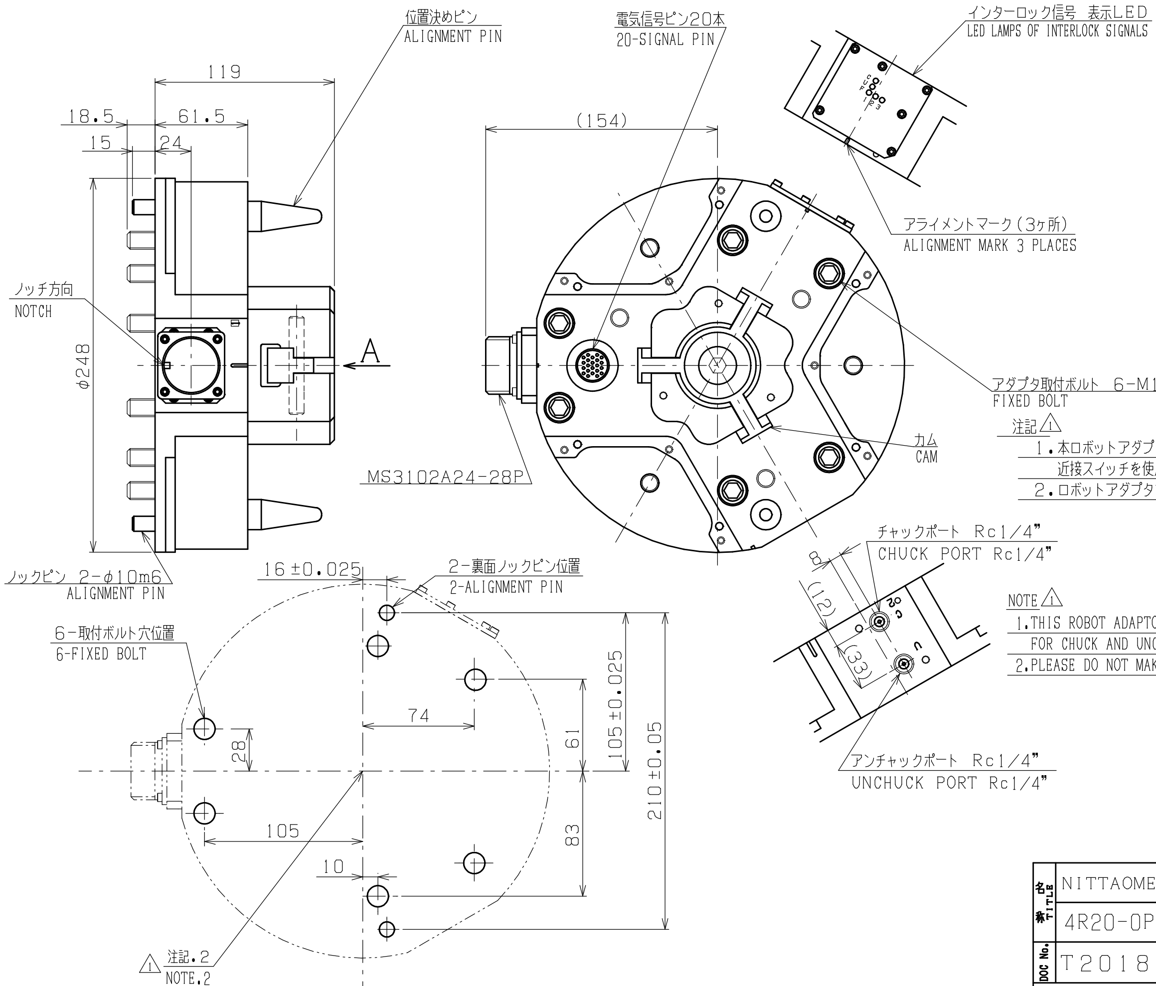
取合寸法図 (A矢視) CONNECTING DIMENSION VIEW (VIEW A)
