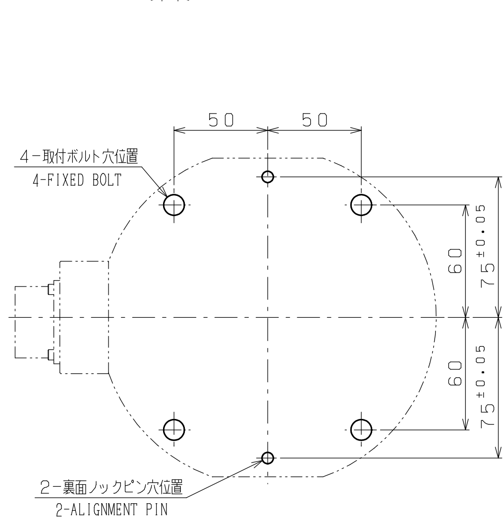
取合寸法図 (A矢視) CONNECTING DIMENSION VIEW (VIEW A)
