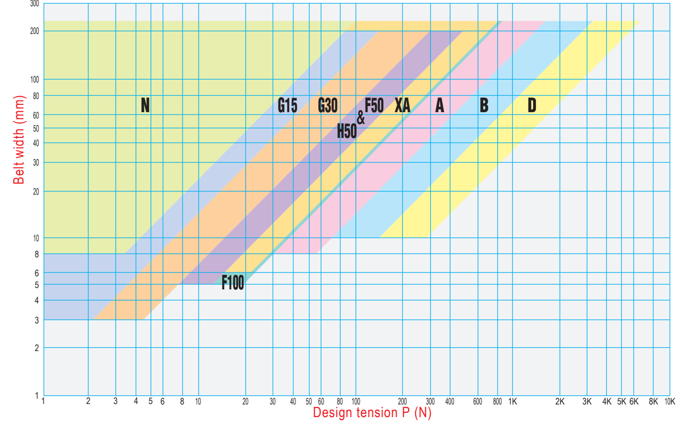
Belt Type Selection Diagram
